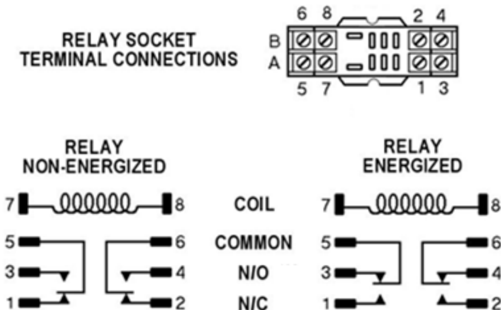
Figure 3-2: Relay Connections
