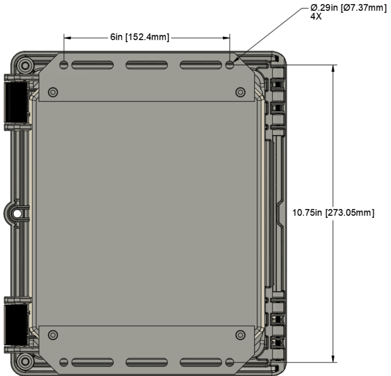
Figure 3-1: Enclosure Mounting
