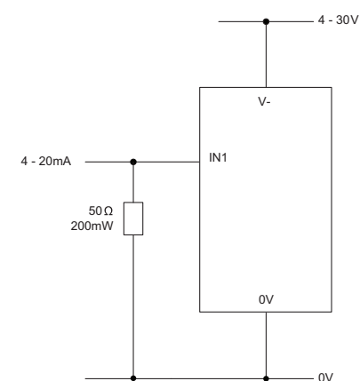
MEASURING 4-20mA
