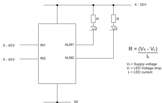
ALARM OUTPUTS
