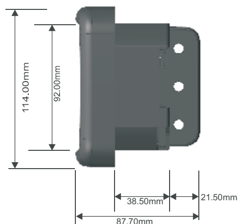
Meter Side View
