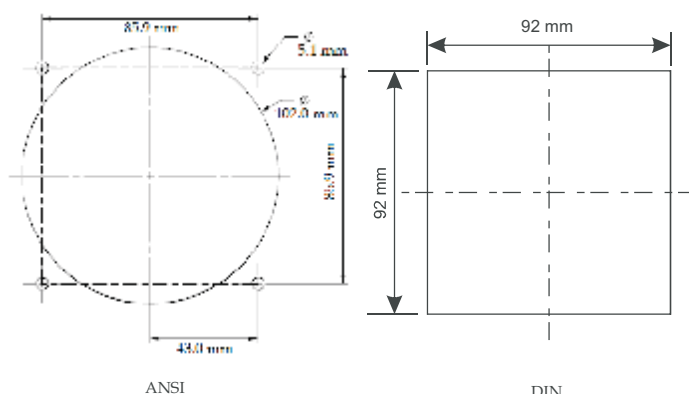
PANEL CUTOUT
