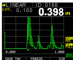
Differential Screen
