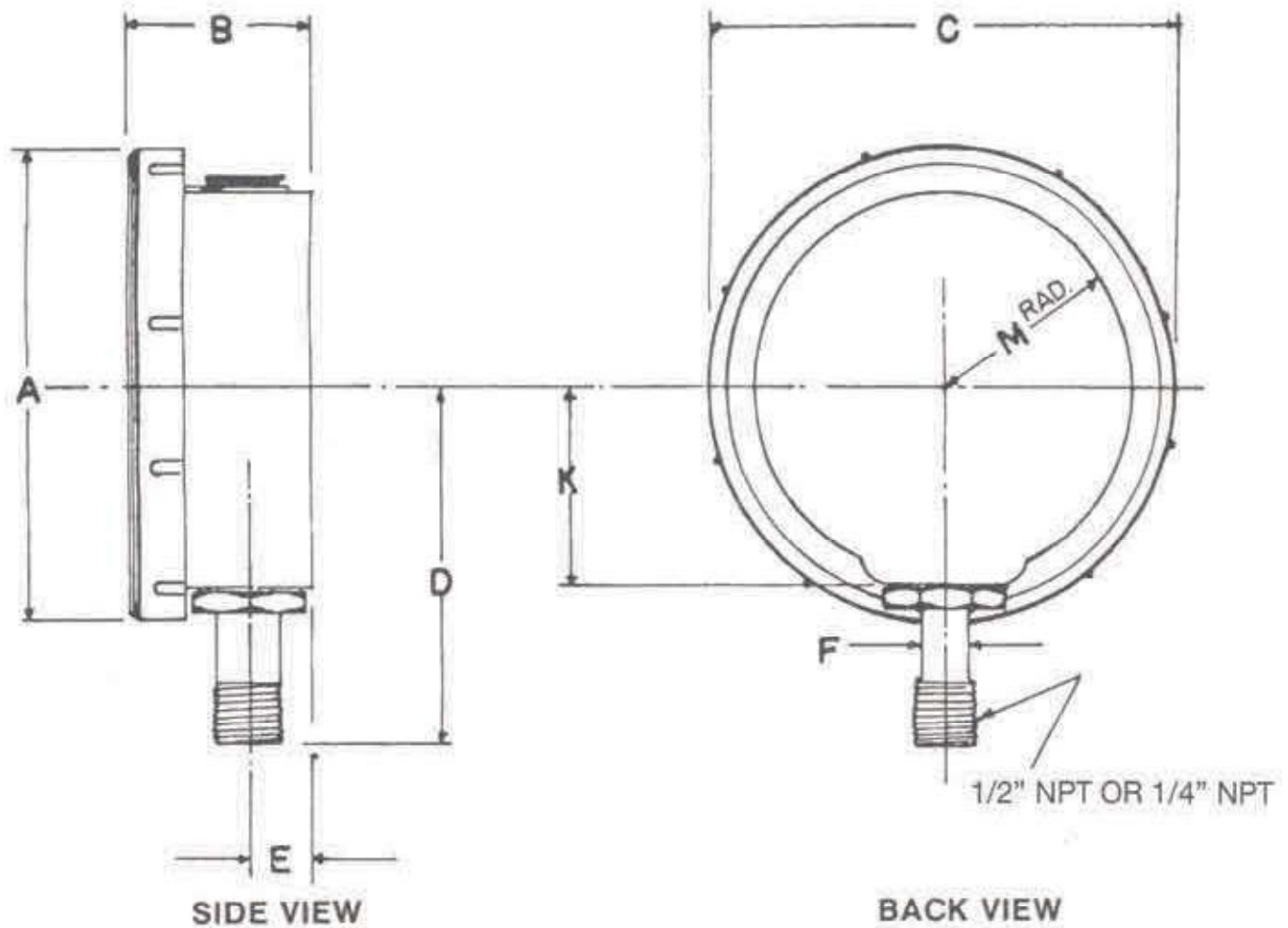
FIG. NO. 901 & 902 SERIES DELRIN
