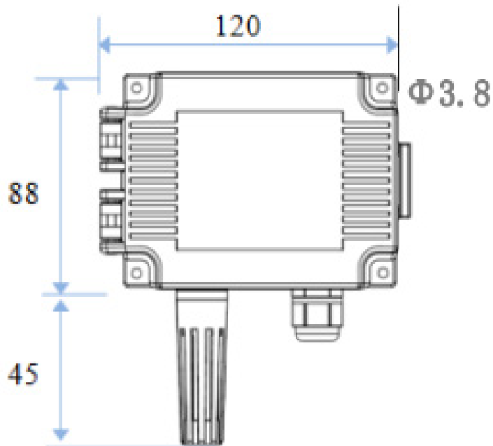
Dimensions (mm)
