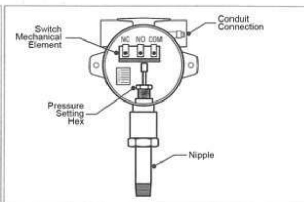
Explosion Proof Type
