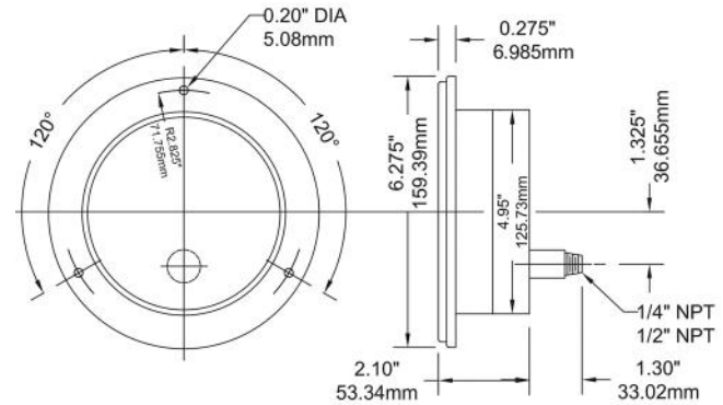
4.5" Back Connection with Front Flange
