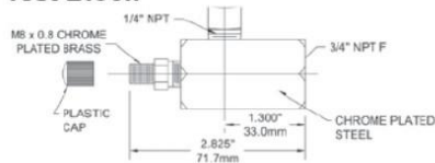
Test Block
